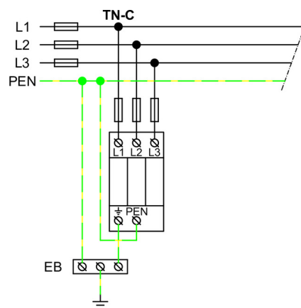
Application wiring diagram (installation)
